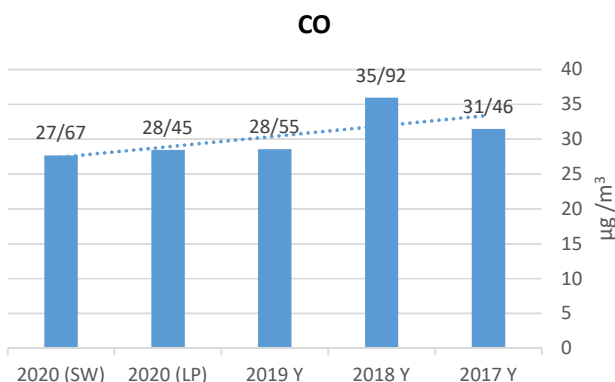
Fig.3 a. Changes in CO concentration in Tehran, LP=Lockdown period, SW=Second wave
